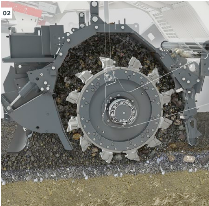
02 - 03 To guarantee optimal mixing results, the WRC 240(i) features a variable mixing chamber like that of the WR Series models.
