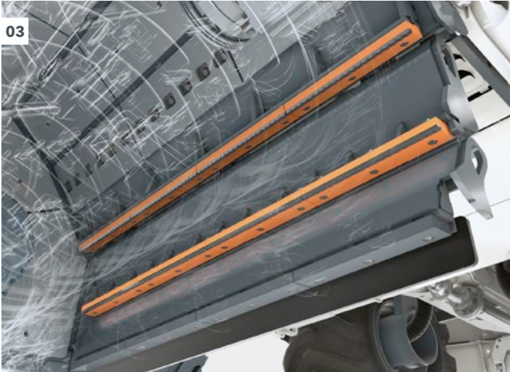
03 The carbide-edged crusher bars of the fixed and variable crushing stage act as counterblades that work in unison with the HT18 crushing tools and enable the rock to be crushed.
