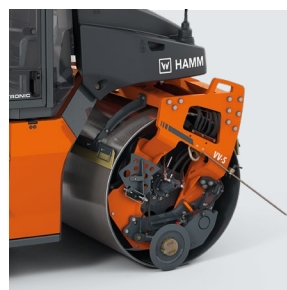
Edge pressing and cutting device
