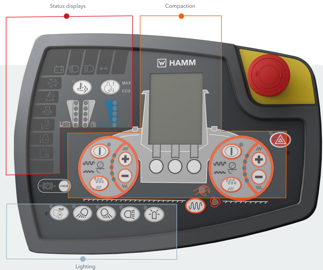
The dashboard next to the steering wheel contains status and parameter displays as well as infrequently used buttons.
